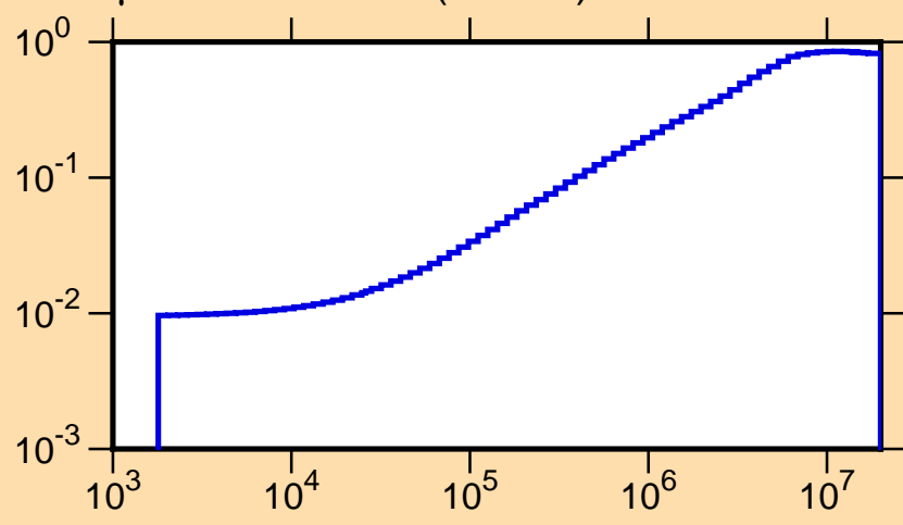
\mu vs. E for ^{71}\text{Cu}(\text{mt251})
