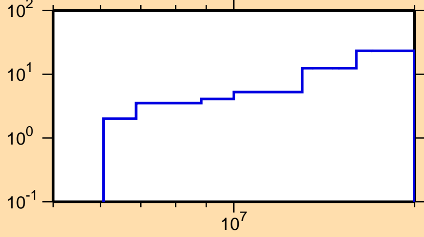
\Delta\sigma/\sigma vs. E for ^{71}\text{Cu}(n,\text{tot.})
