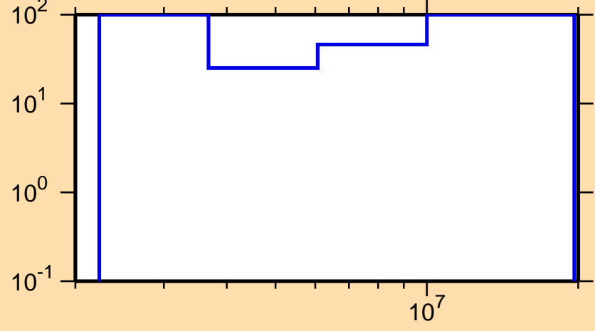
\Delta\sigma/\sigma vs. E for ^{71}\text{Cu}(n,n\text{cont.})
