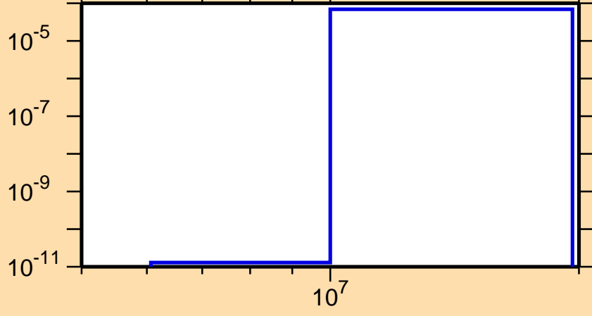
\sigma vs. E for ^{71}\text{Cu}(n,\alpha)
