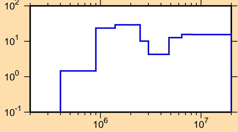
\Delta\sigma/\sigma vs. E for ^{71}\text{Cu}(n,\text{el.})
