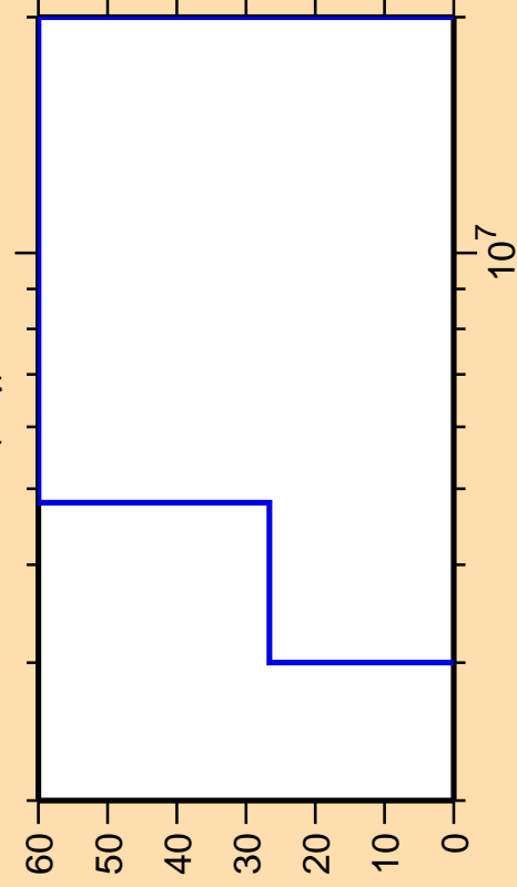
\Delta\sigma/\sigma vs. E for ^{71}\text{Cu}(n,\gamma)
