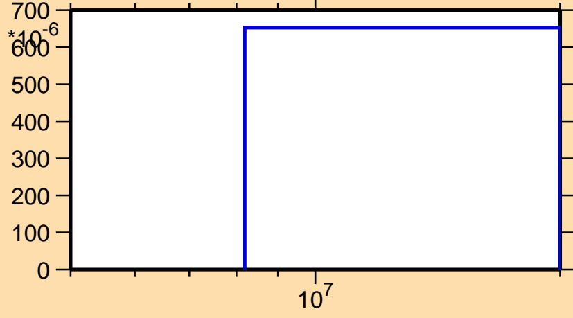
\sigma vs. E for ^{71}\text{Cu}(n,d)
