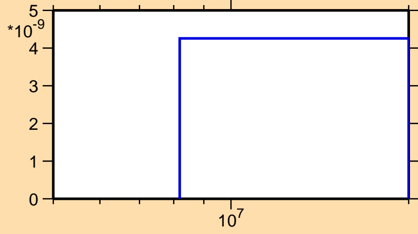
\sigma vs. E for ^{71}\text{Cu}(n,\text{nd})
