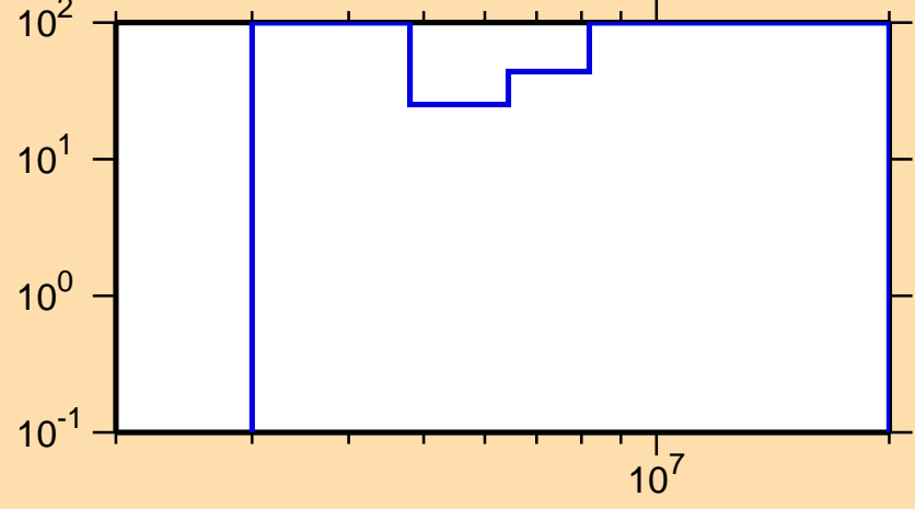
\Delta\sigma/\sigma vs. E for ^{71}\text{Cu}(n,ncont.)
