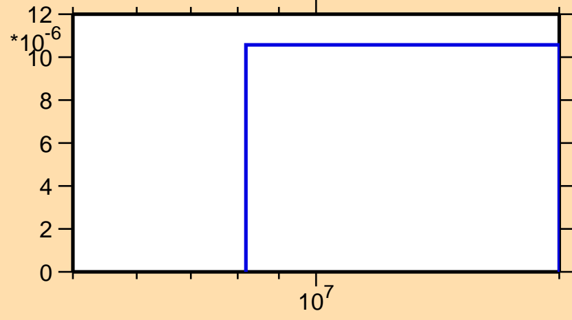
\sigma vs. E for ^{71}\text{Cu}(n,t)
