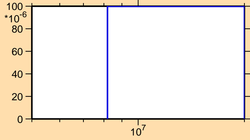
\sigma vs. E for ^{71}\text{Cu}(n,np)
