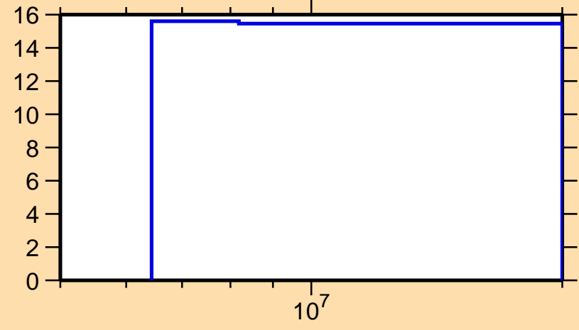
\Delta\sigma/\sigma vs. E for ^{71}\text{Cu}(n,el.)
