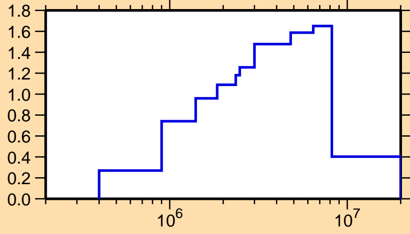
\sigma vs. E for ^{71}\text{Cu}(n,\text{inel.})
