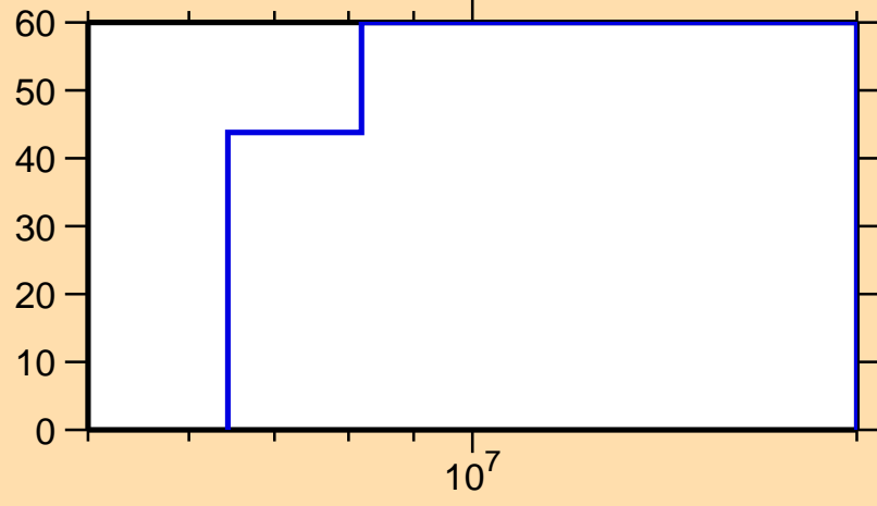
\Delta\sigma/\sigma vs. E for ^{71}\text{Cu}(n,n\text{cont.})
