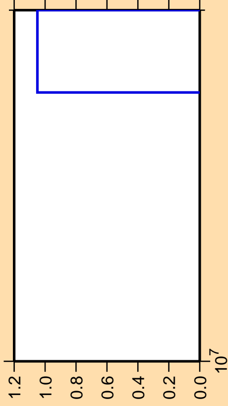
\Delta\sigma/\sigma vs. E for ^{73}\text{Cu}(n,2np)
