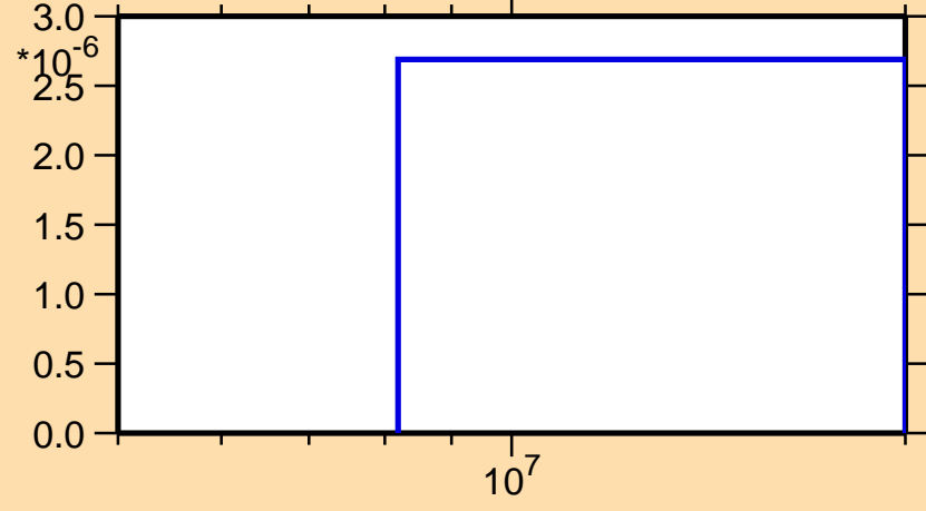
\sigma vs. E for ^{73}\text{Cu}(n,t)
