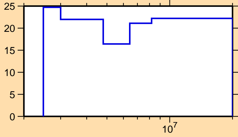
\Delta\sigma/\sigma vs. E for ^{73}\text{Cu}(n,n\text{nonel.})
