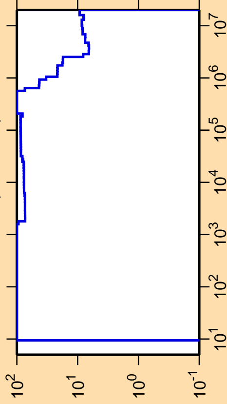
\Delta\sigma/\sigma vs. E for ^{74}\text{Cu}(n,\text{nonel.})
