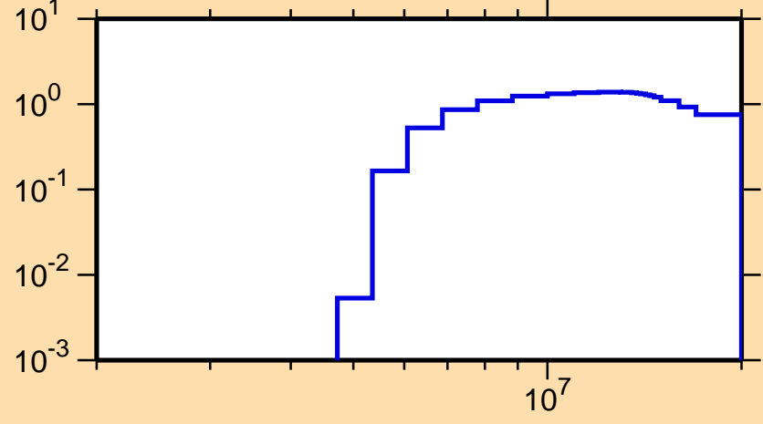
\sigma vs. E for ^{74}\text{Cu}(n,2n)
