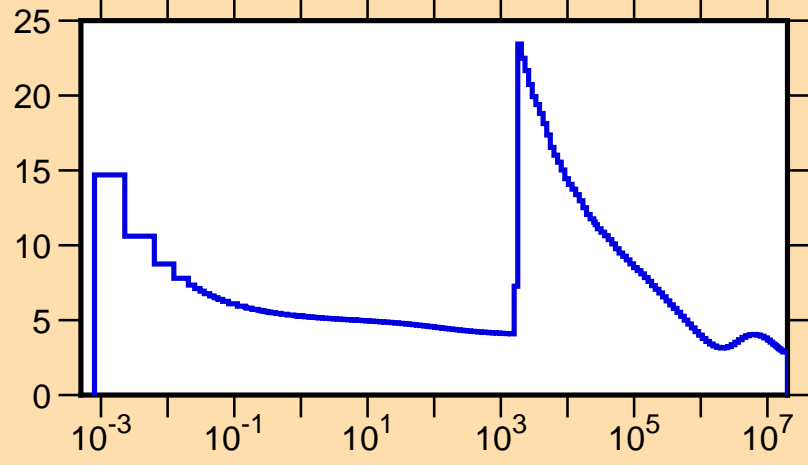
\sigma vs. E for ^{74}\text{Cu}(n,\text{tot.})
