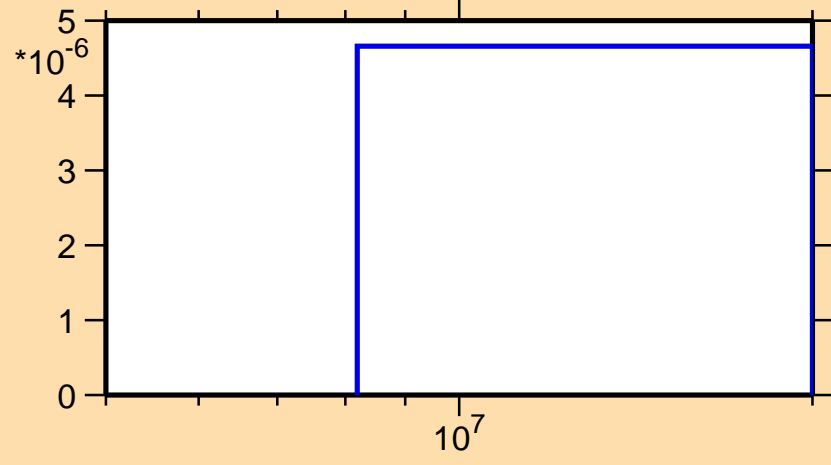
\sigma vs. E for ^{74}\text{Cu}(n,np)
