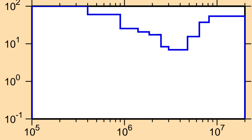
\Delta\sigma/\sigma vs. E for ^{74}\text{Cu}(n,\text{inel.})
