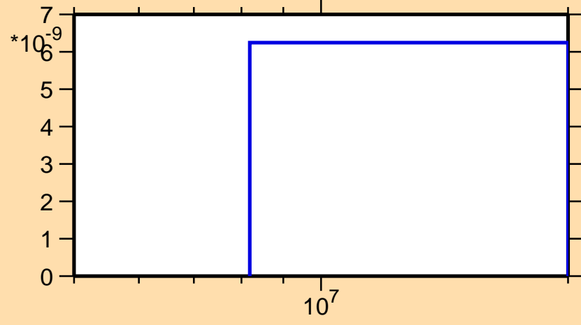
\sigma vs. E for ^{74}\text{Cu}(n,\alpha)
