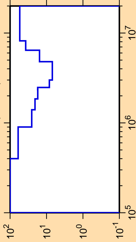
\Delta\sigma/\sigma vs. E for ^{74}\text{Cu}(n,\text{inel.})
