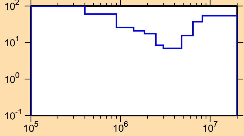
\Delta\sigma/\sigma vs. E for ^{74}\text{Cu}(n,n\text{cont.})
