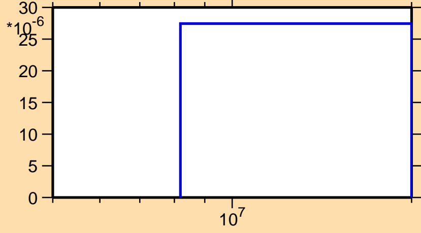
\sigma vs. E for ^{74}\text{Cu}(n,t)
