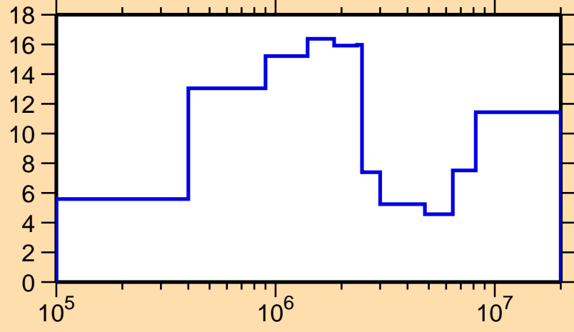
\Delta\sigma/\sigma vs. E for ^{74}\text{Cu}(n,tot.)
