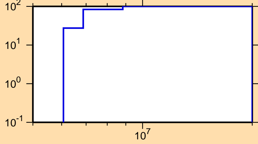
\Delta\sigma/\sigma vs. E for ^{75}\text{Cu}(n,\text{inel.})
