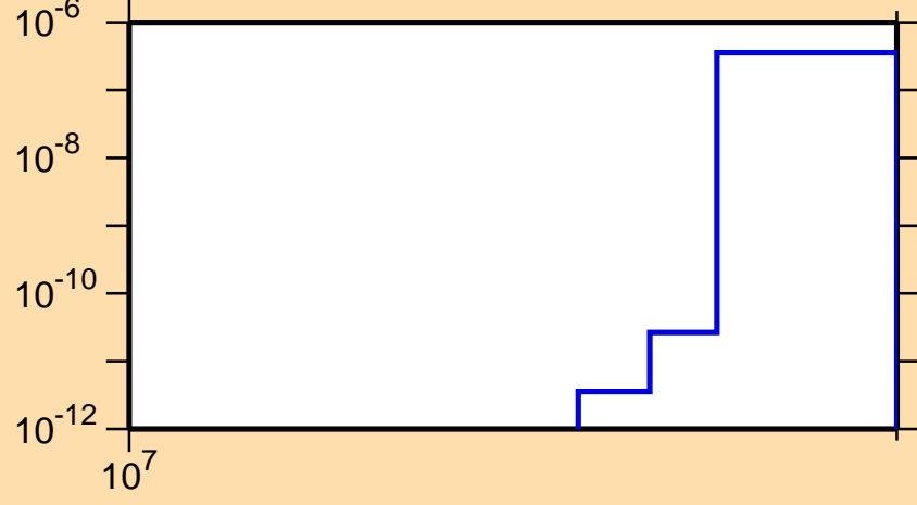
\sigma vs. E for ^{75}\text{Cu}(n,nt)
