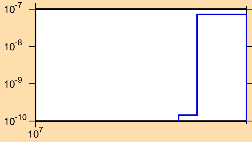
\sigma vs. E for ^{75}\text{Cu}(n,\alpha)
