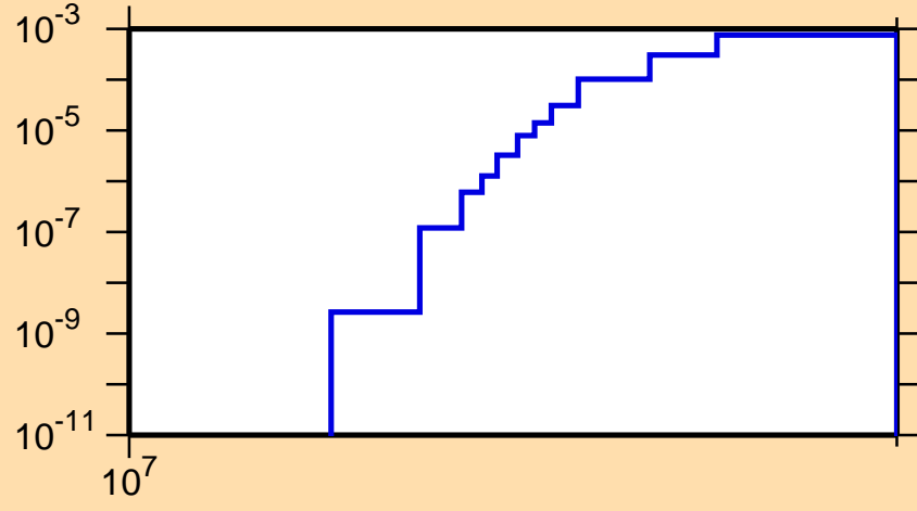
\sigma vs. E for ^{75}\text{Cu}(n,d)
