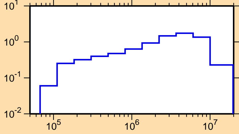
\sigma vs. E for ^{75}\text{Cu}(n,\text{inel.})
