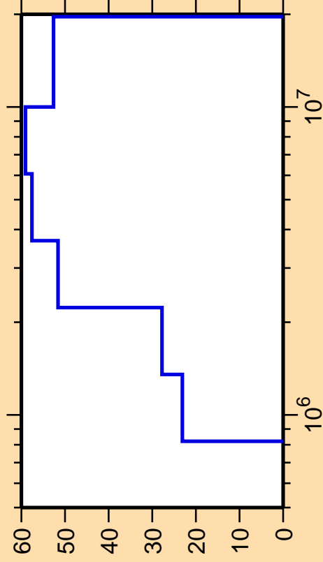
\Delta\sigma/\sigma vs. E for ^{75}\text{Cu}(n,n_3)
