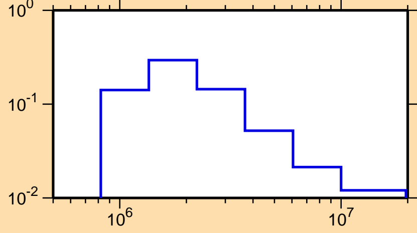
\sigma vs. E for ^{75}\text{Cu}(n,n_3)
