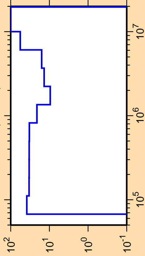
\Delta\sigma/\sigma vs. E for ^{75}\text{Cu}(n,\text{inel.})
