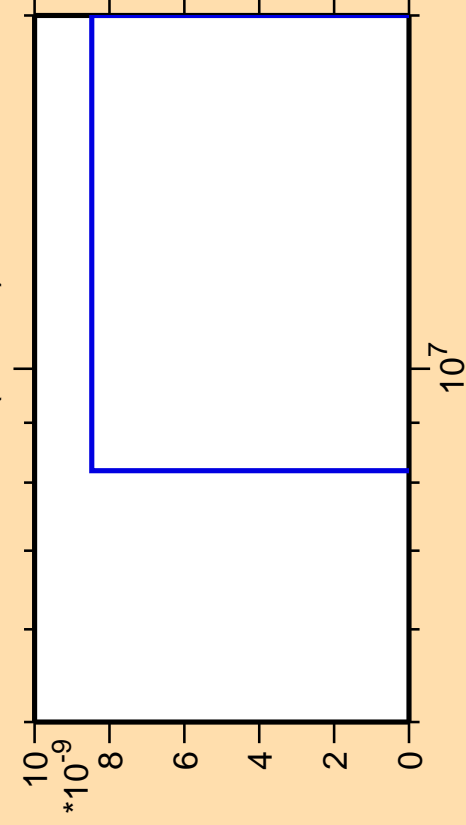
\Delta\sigma/\sigma vs. E for ^{75}\text{Cu}(n,2n\alpha)
