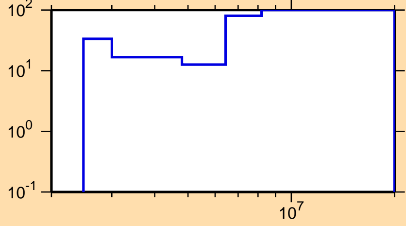
\Delta\sigma/\sigma vs. E for ^{75}\text{Cu}(n,n\text{cont.})
