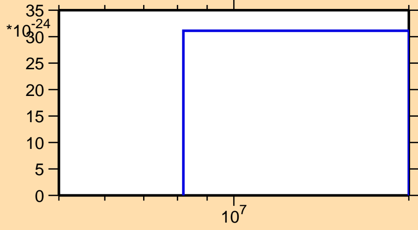
\sigma vs. E for ^{75}\text{Cu}(n,2np)
