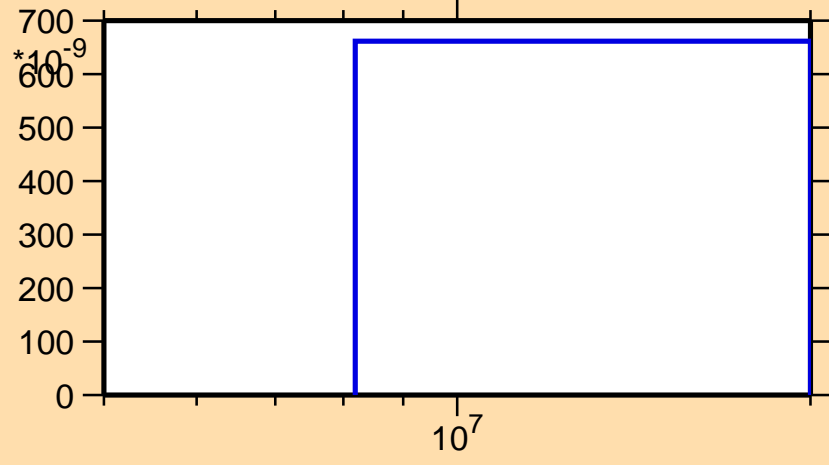
\sigma vs. E for ^{75}\text{Cu}(n,t)
