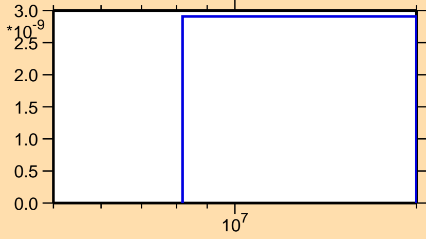
\sigma vs. E for ^{75}\text{Cu}(n,nt)
