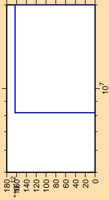
\Delta\sigma/\sigma vs. E for ^{75}\text{Cu}(n,2np)
