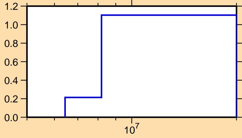
\sigma vs. E for ^{75}\text{Cu}(n,2n)
