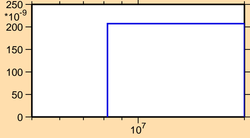
\sigma vs. E for ^{75}\text{Cu}(n,\alpha)
