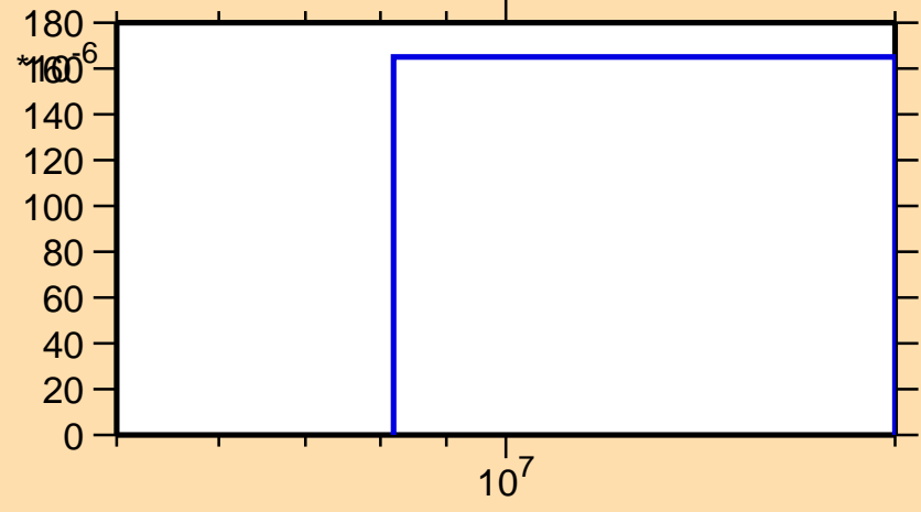
\sigma vs. E for ^{75}\text{Cu}(n,p)
