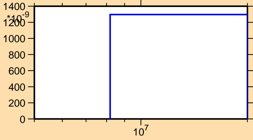
\sigma vs. E for ^{75}\text{Cu}(n,np)
