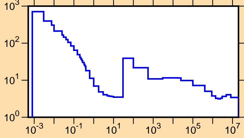
\sigma vs. E for ^{76}\text{Cu}(n,\text{tot.})
