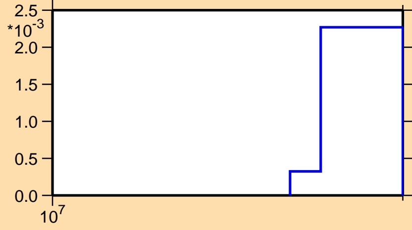
\sigma vs. E for ^{256}\alpha )
