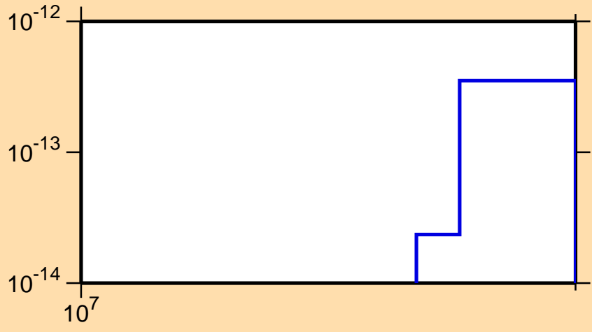
\sigma vs. E for ^{260}
