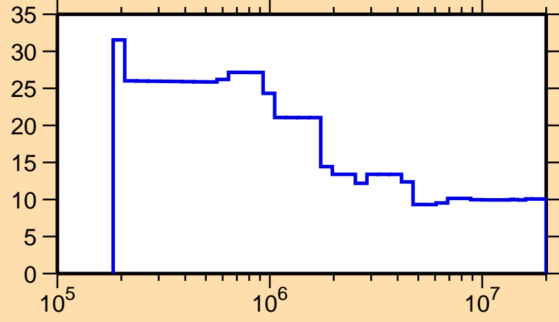
\Delta\sigma/\sigma vs. E for ^{260}
