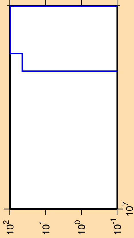
\Delta\sigma/\sigma vs. E for ^{260}
