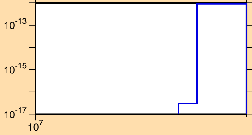
\sigma vs. E for ^{263}
