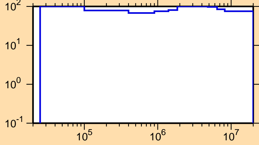
\Delta\sigma/\sigma vs. E for ^{263}_1 )
