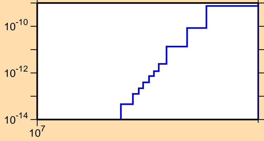
\sigma vs. E for ^{267}\text{He3} )
