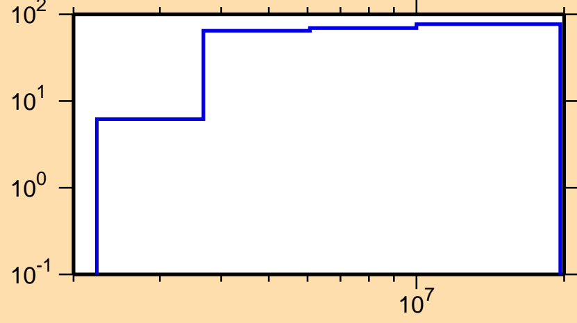
\Delta\sigma/\sigma vs. E for ^{267}
