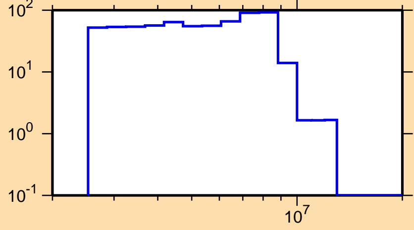
\Delta\sigma/\sigma vs. E for ^{270}_1
