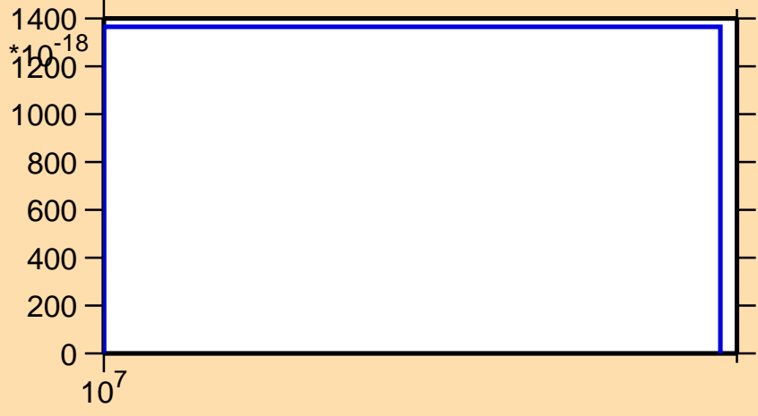
\sigma vs. E for ^{280}
