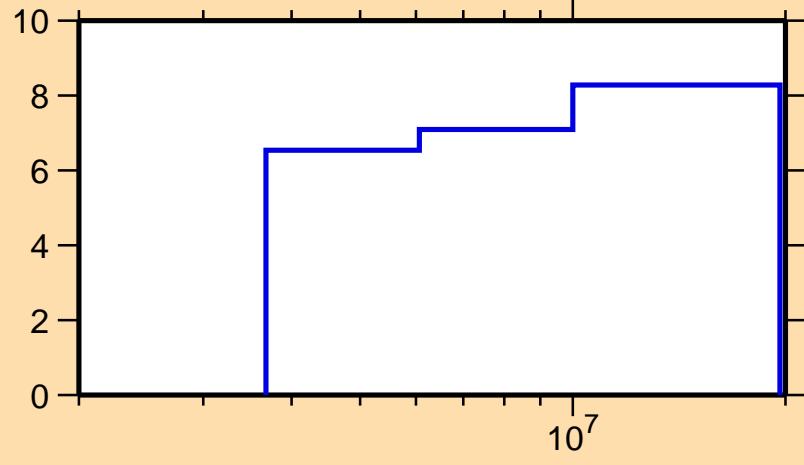
\Delta\sigma/\sigma vs. E for ^{17}\text{F}(n,n\text{onel.})
