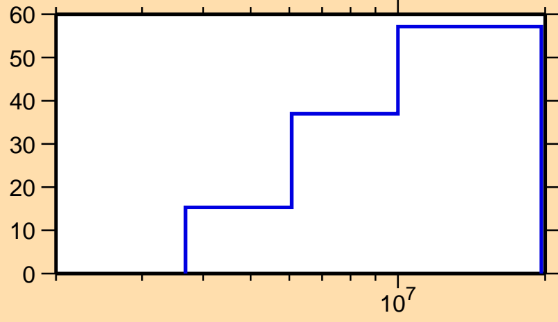
\Delta\sigma/\sigma vs. E for ^{17}\text{F}(n,inel.)
