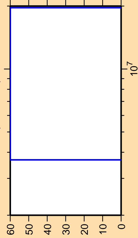
\Delta\sigma/\sigma vs. E for ^{17}\text{F}(n,ncont.)
