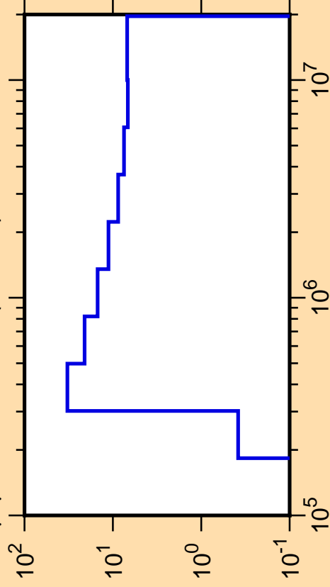
\Delta\mu/\mu vs. E for ^{21}\text{F}(\text{mt251})
