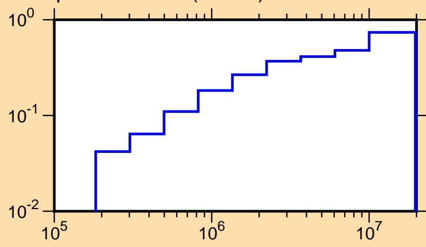
\mu vs. E for ^{21}\text{F}(\text{mt251})
