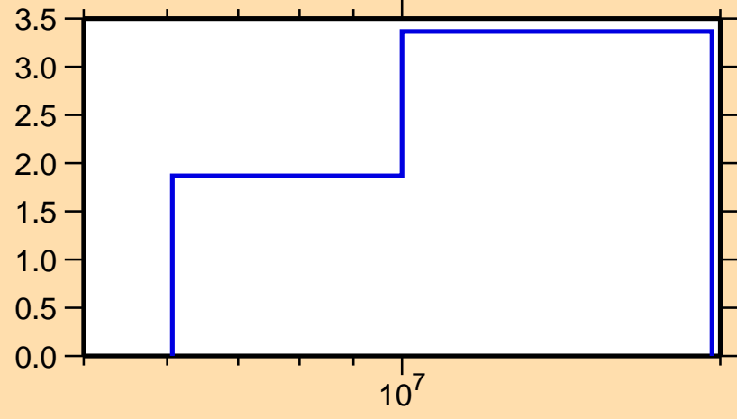
\Delta\sigma/\sigma vs. E for ^{21}\text{F}(n,n\text{onel.})
