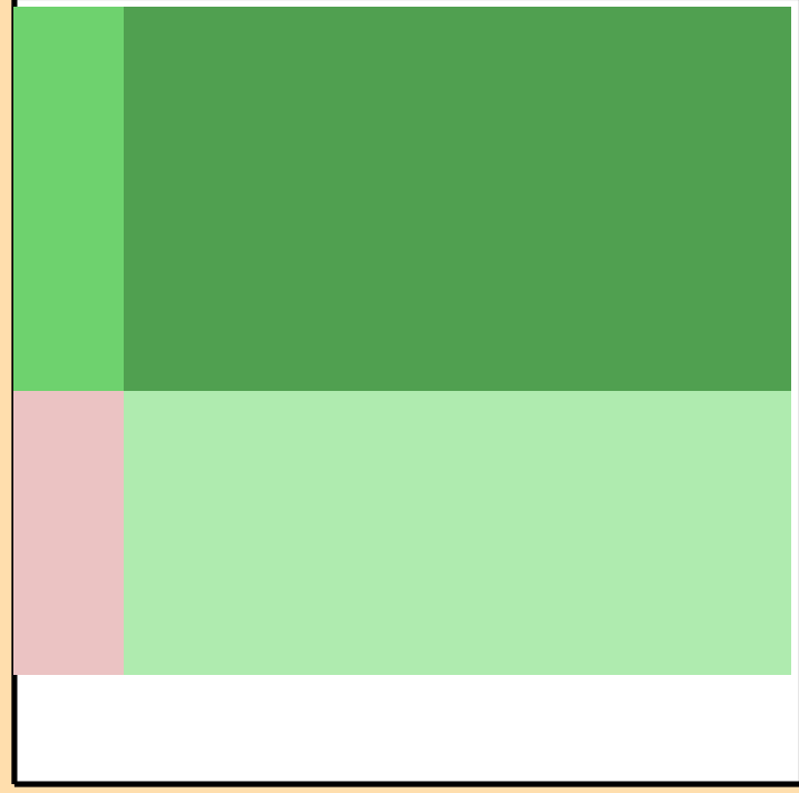
\Delta\sigma/\sigma vs. E for ^{21}\text{F}(n,\gamma)
