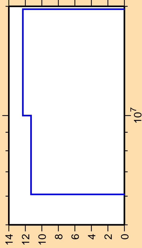
\Delta\sigma/\sigma vs. E for ^{21}\text{F}(n,\text{ncont.})
