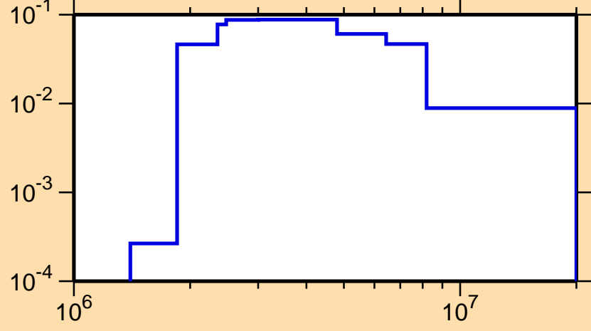
\sigma vs. E for ^{21}\text{F}(n,n_3)
