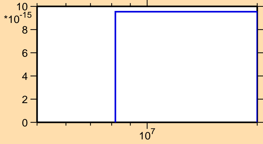
\sigma vs. E for ^{21}\text{F}(n,2np)
