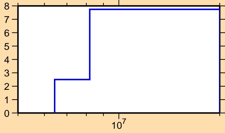
\Delta\sigma/\sigma vs. E for ^{21}\text{F}(n,el.)
