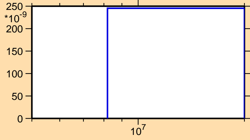
\sigma vs. E for ^{21}\text{F}(n,nd)
