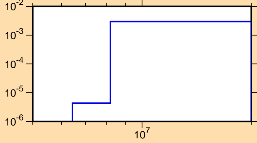
\sigma vs. E for ^{21}\text{F}(n,p)
