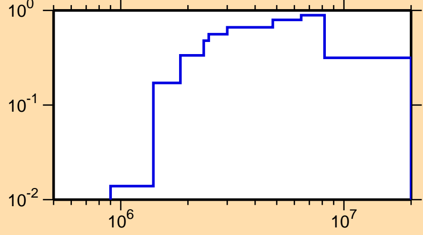
\sigma vs. E for ^{21}\text{F}(n,\text{inel.})
