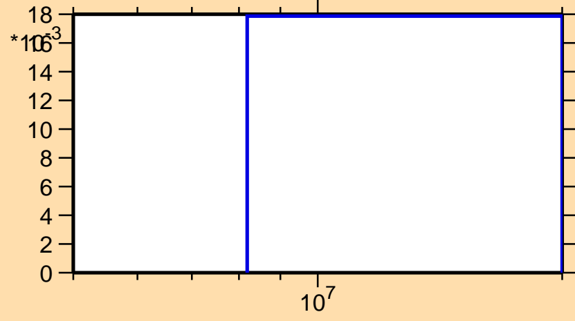
\sigma vs. E for ^{21}\text{F}(n,d)
