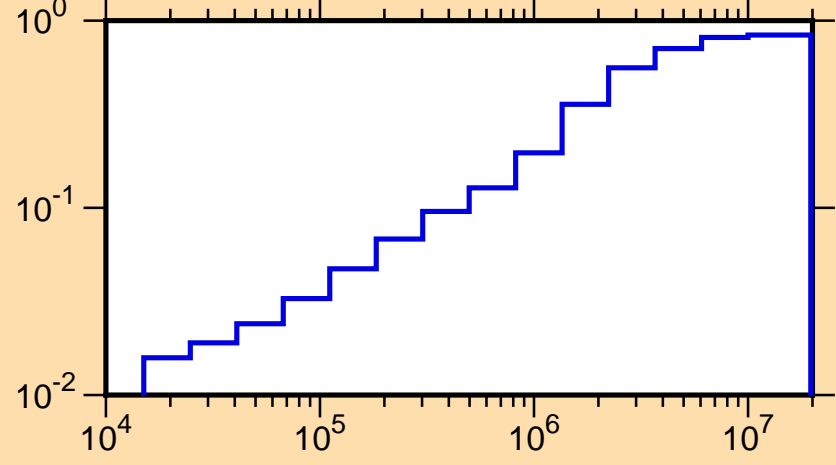
\mu vs. E for ^{52}\text{Fe}(\text{mt251})
