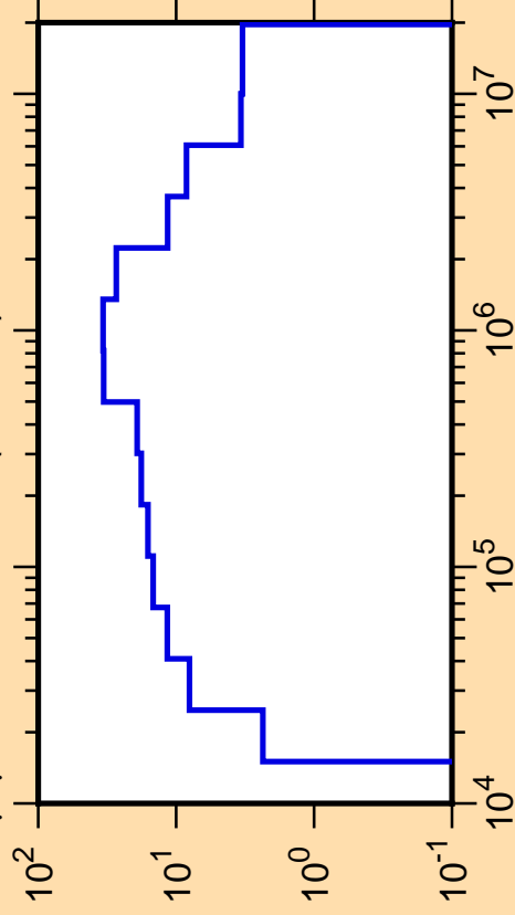
\Delta\mu/\mu vs. E for ^{52}\text{Fe}(\text{mt251})
