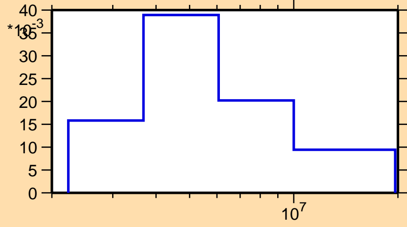
\sigma vs. E for ^{52}\text{Fe}(n,n_2)
