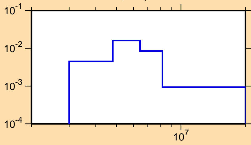
\sigma vs. E for ^{52}\text{Fe}(n,n_4)
