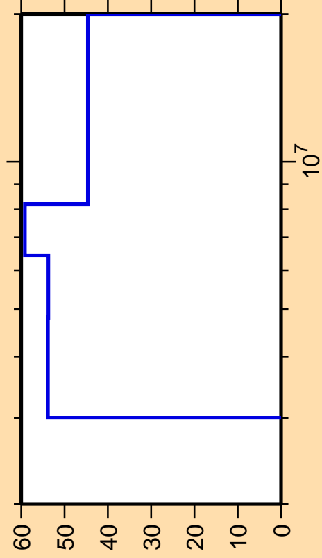
\Delta\sigma/\sigma vs. E for ^{52}\text{Fe}(n,n_4)
