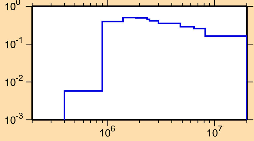
\sigma vs. E for ^{52}\text{Fe}(n,\text{inel.})
