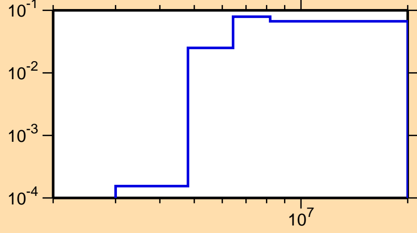
\sigma vs. E for ^{52}\text{Fe}(n,n\text{cont.})
