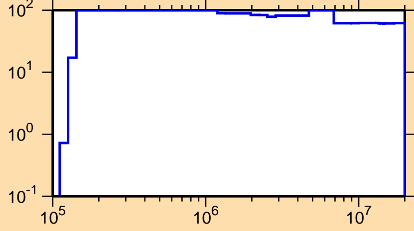
\Delta\sigma/\sigma vs. E for ^{52}\text{Fe}(n,n\text{cont.})
