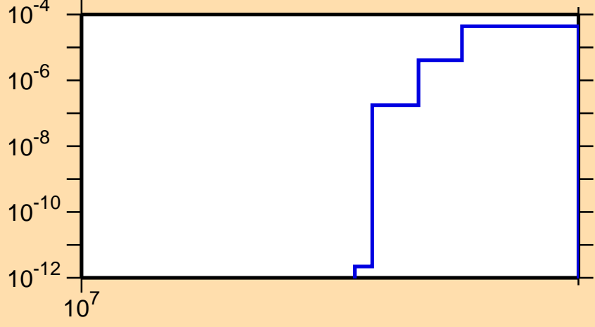
\sigma vs. E for ^{52}\text{Fe}(n,2np)
