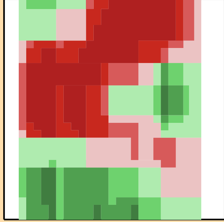
\Delta\sigma/\sigma vs. E for ^{52}\text{Fe}(n,n_1)
