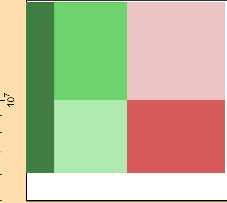
\Delta\sigma/\sigma vs. E for ^{52}\text{Fe}(n,\text{tot.})
