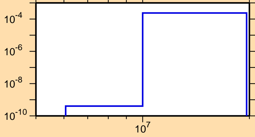
\sigma vs. E for ^{52}\text{Fe}(n,2n)
