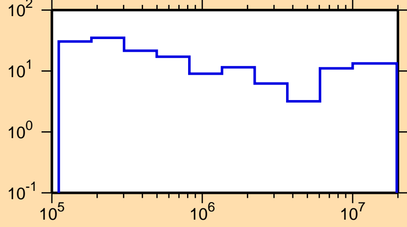
\Delta\sigma/\sigma vs. E for ^{52}\text{Fe}(n,\text{tot.})
