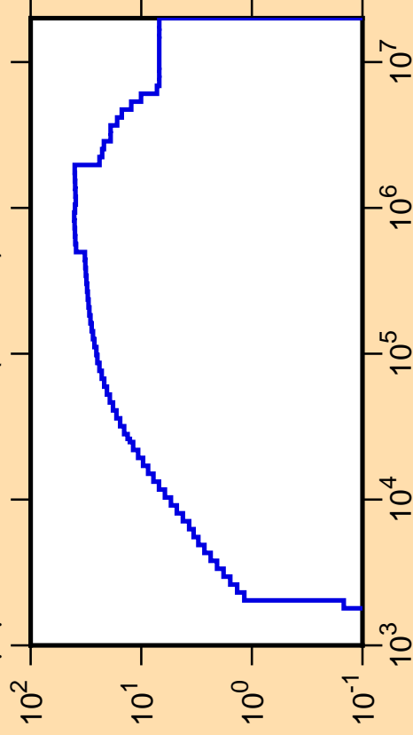
\Delta\mu/\mu vs. E for ^{53}\text{Fe}(\text{mt251})
