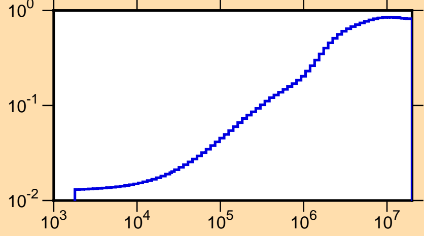
\mu vs. E for ^{53}\text{Fe}(\text{mt251})
