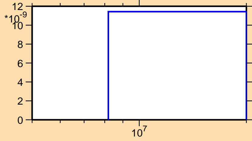
\sigma vs. E for ^{53}\text{Fe}(n,nd)
