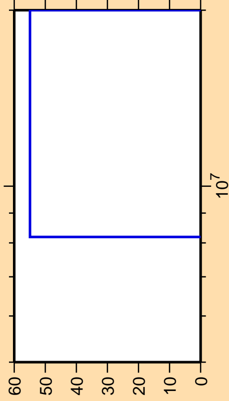
\Delta\sigma/\sigma vs. E for ^{53}\text{Fe}(n,nd)
