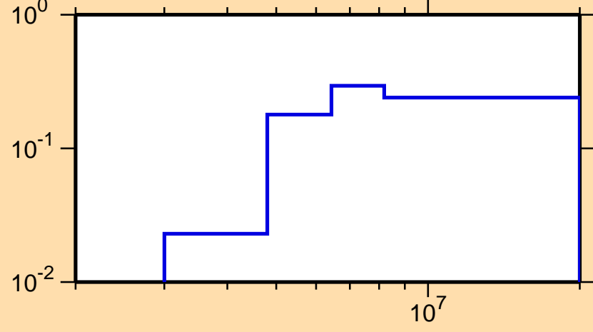
\sigma vs. E for ^{53}\text{Fe}(n,n\text{cont.})
