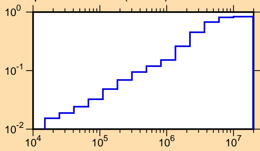
\mu vs. E for ^{54}\text{Fe}(\text{mt251})
