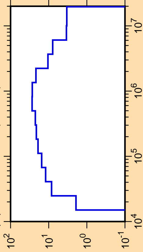
\Delta\mu/\mu vs. E for ^{54}\text{Fe}(\text{mt251})
