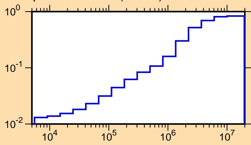
\mu vs. E for ^{55}\text{Fe}(\text{mt251})
