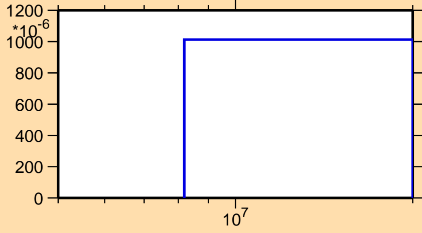
\sigma vs. E for ^{55}\text{Fe}(n,\alpha)
