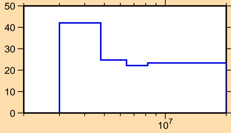
\Delta\sigma/\sigma vs. E for ^{55}\text{Fe}(n,n\text{cont.})
