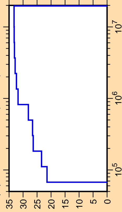
\Delta\mu/\mu vs. E for ^{56}\text{Fe}(\text{mt251})
