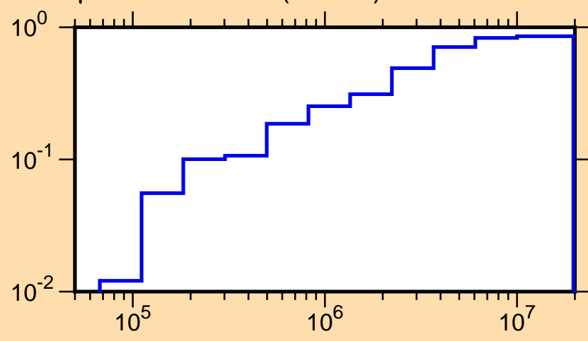
\mu vs. E for ^{56}\text{Fe}(\text{mt251})
