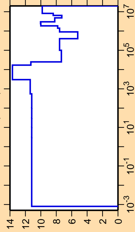
\Delta\sigma/\sigma vs. E for ^{56}\text{Fe}(n,\text{el.})
