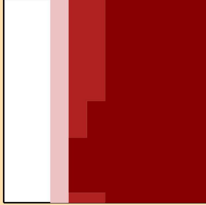
\Delta\sigma/\sigma vs. E for ^{57}\text{Fe}(n,2n)
