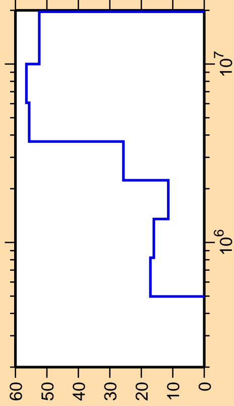
\Delta\sigma/\sigma vs. E for ^{57}\text{Fe}(n,n_4)
