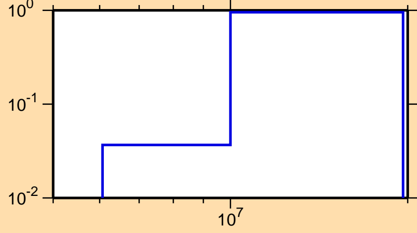
\sigma vs. E for ^{57}\text{Fe}(n,2n)
