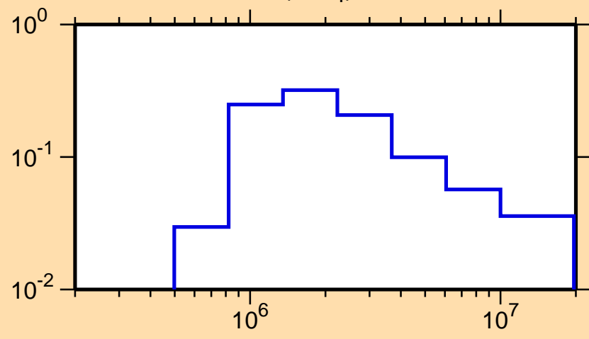
\sigma vs. E for ^{57}\text{Fe}(n,n_4)
