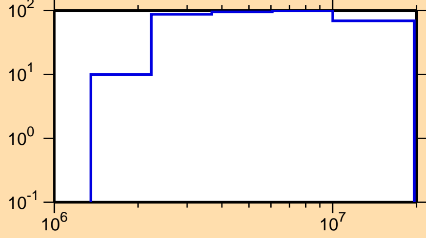
\Delta\sigma/\sigma vs. E for ^{57}\text{Fe}(n,p)
