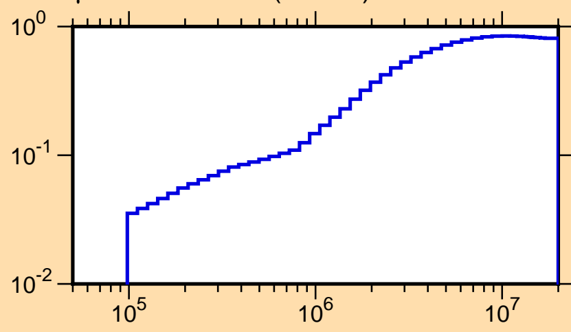
\mu vs. E for ^{58}\text{Fe}(\text{mt251})
