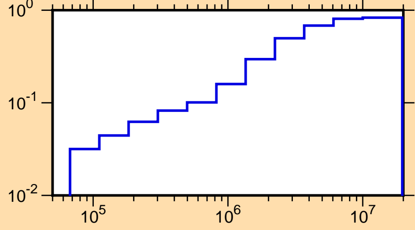
\mu vs. E for ^{58}\text{Fe}(\text{mt251})
