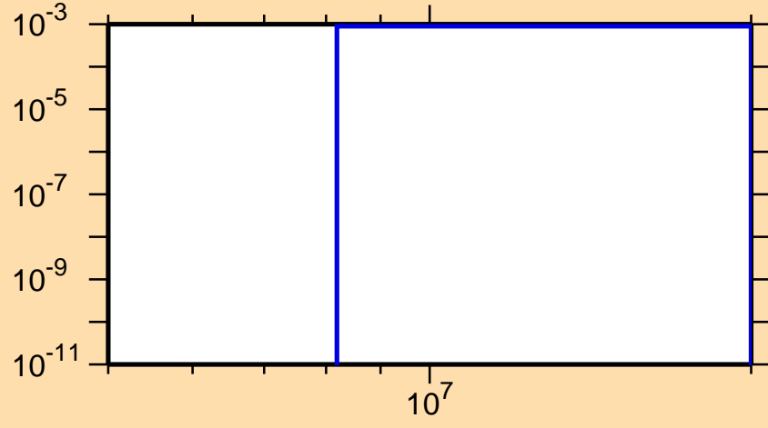
\sigma vs. E for ^{58}\text{Fe}(n,\alpha)
