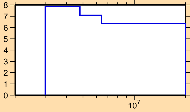
\Delta\sigma/\sigma vs. E for ^{58}\text{Fe}(n,n\text{onel.})
