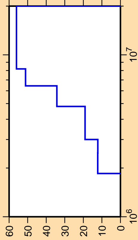
\Delta\sigma/\sigma vs. E for ^{58}\text{Fe}(n,n_4)
