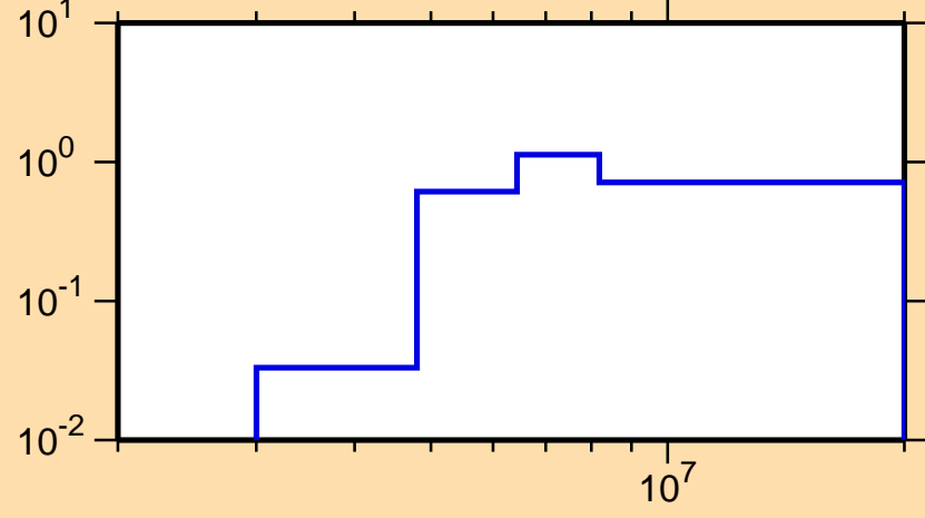
\sigma vs. E for ^{58}\text{Fe}(n,n\text{cont.})
