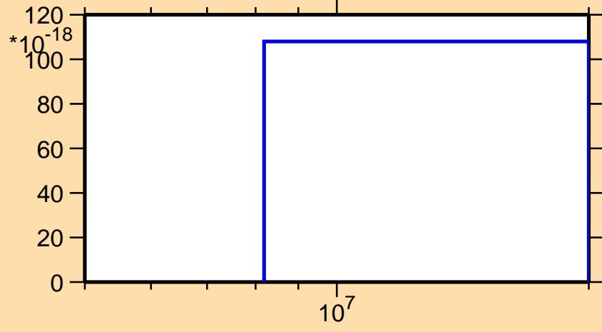
\sigma vs. E for ^{58}\text{Fe}(n,nt)
