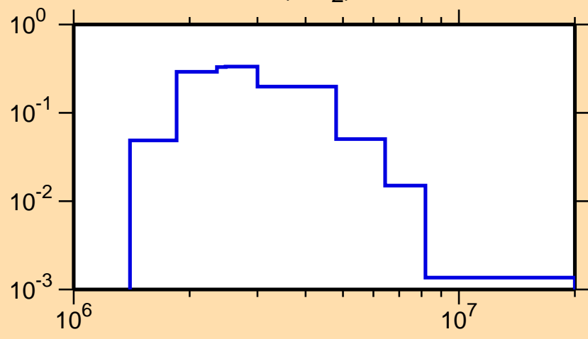
\sigma vs. E for ^{58}\text{Fe}(n,n_2)
