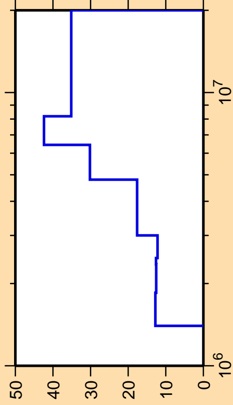
\Delta\sigma/\sigma vs. E for ^{58}\text{Fe}(n,n_2)
