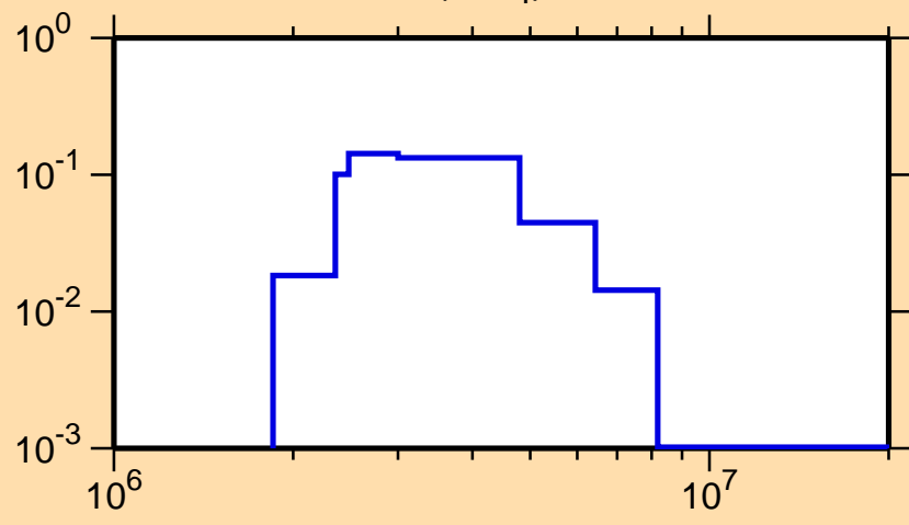
\sigma vs. E for ^{58}\text{Fe}(n,n_4)
