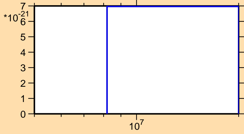
\sigma vs. E for ^{58}\text{Fe}(n,pd)
