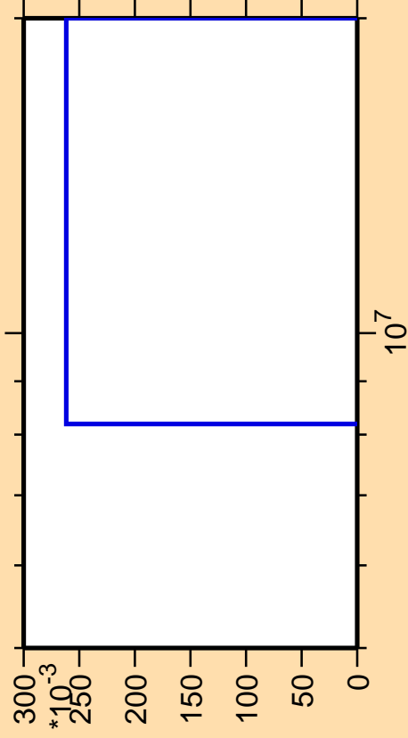
\Delta\sigma/\sigma vs. E for ^{58}\text{Fe}(n,nd)
