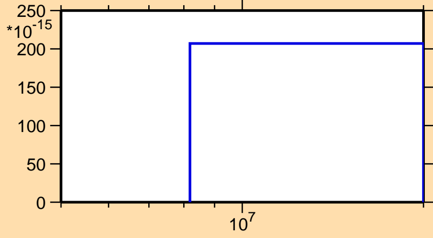
\sigma vs. E for ^{58}\text{Fe}(n,nd)
