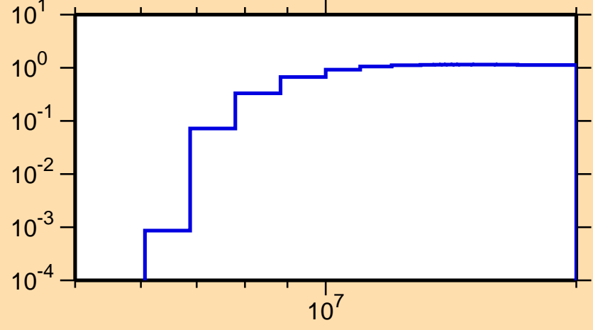
\sigma vs. E for ^{59}\text{Fe}(n,2n)
