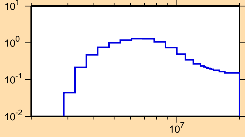
\sigma vs. E for ^{59}\text{Fe}(n,n\text{cont.})
