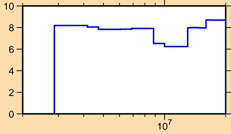
\Delta\sigma/\sigma vs. E for ^{59}\text{Fe}(n,n\text{onel.})
