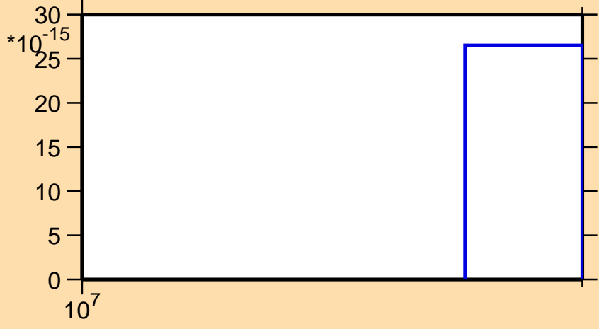
\sigma vs. E for ^{59}\text{Fe}(n,nt)
