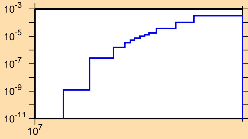
\sigma vs. E for ^{59}\text{Fe}(n,t)
