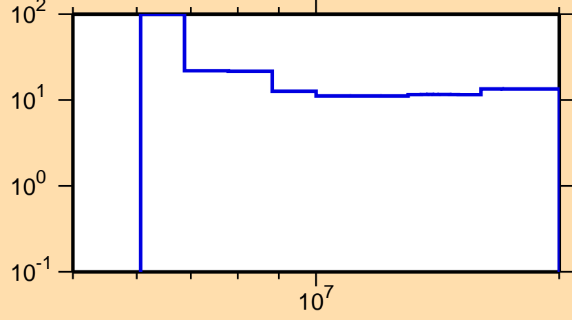
\Delta\sigma/\sigma vs. E for ^{59}\text{Fe}(n,2n)
