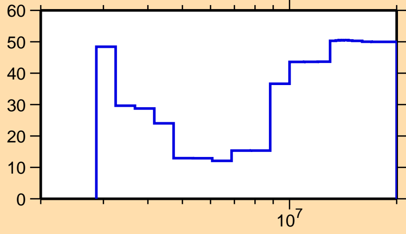
\Delta\sigma/\sigma vs. E for ^{59}\text{Fe}(n,ncont.)
