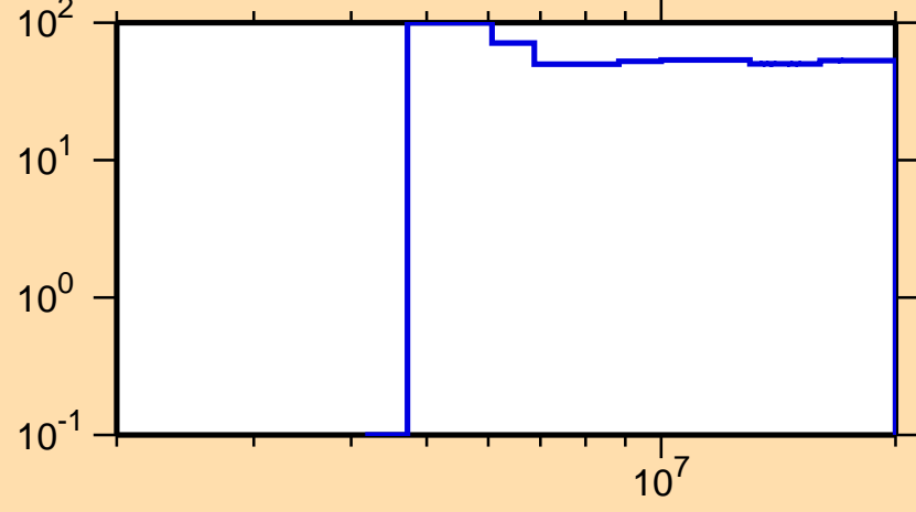
\Delta\sigma/\sigma vs. E for ^{59}\text{Fe}(n,p)
