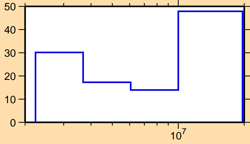
\Delta\sigma/\sigma vs. E for ^{59}\text{Fe}(n,n\text{cont.})
