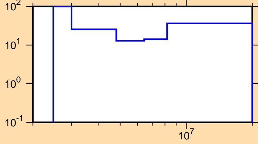
\Delta\sigma/\sigma vs. E for ^{59}\text{Fe}(n,n\text{cont.})
