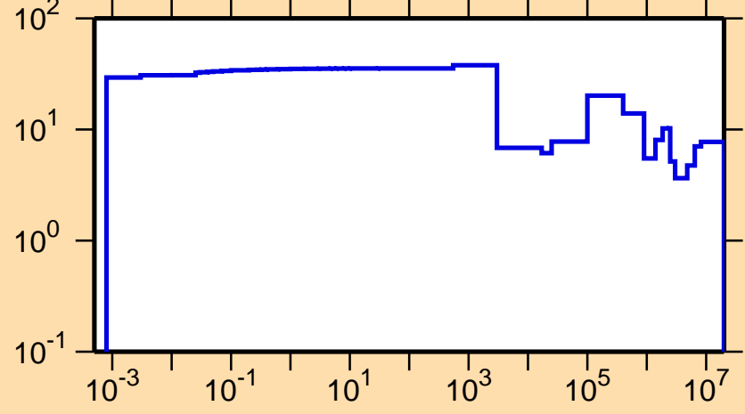
\Delta\sigma/\sigma vs. E for ^{59}\text{Fe}(n,\text{tot.})
