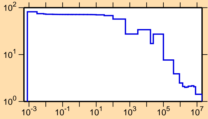
\sigma vs. E for ^{59}\text{Fe}(n,\text{el.})
