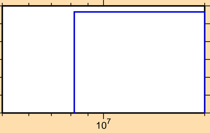
\sigma vs. E for ^{59}\text{Fe}(n,np)
