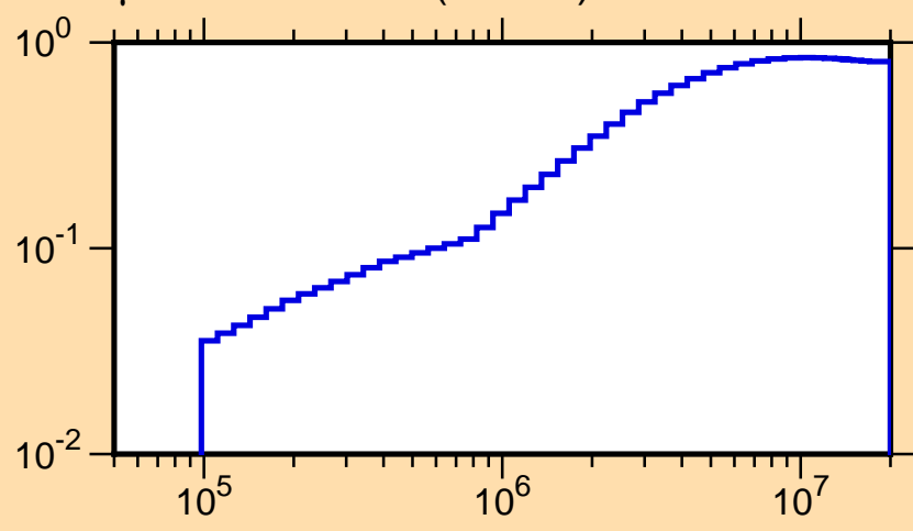
\mu vs. E for ^{60}\text{Fe}(\text{mt251})
