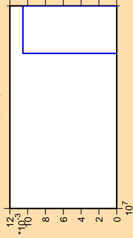
\Delta\sigma/\sigma vs. E for ^{60}\text{Fe}(n,nt)
