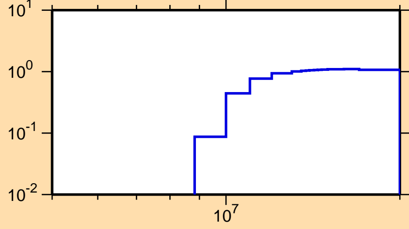
\sigma vs. E for ^{60}\text{Fe}(n,2n)
