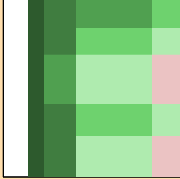
\Delta\sigma/\sigma vs. E for ^{61}\text{Fe}(n,p)
