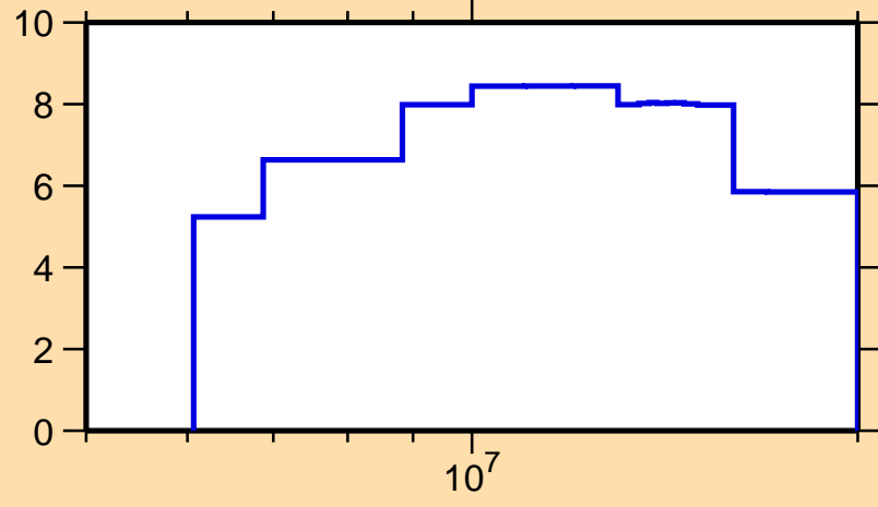
\Delta\sigma/\sigma vs. E for ^{61}\text{Fe}(n,el.)
