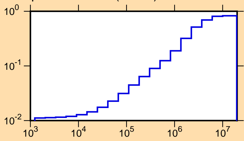
\mu vs. E for ^{61}\text{Fe}(\text{mt251})
