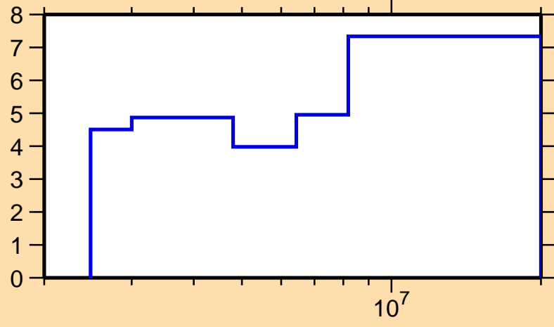
\Delta\sigma/\sigma vs. E for ^{61}\text{Fe}(n,\text{inel.})
