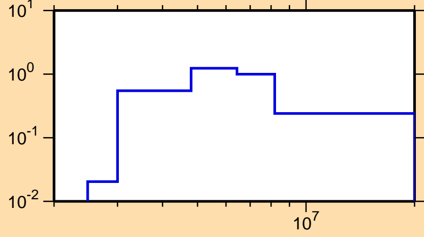
\sigma vs. E for ^{61}\text{Fe}(n,n\text{cont.})
