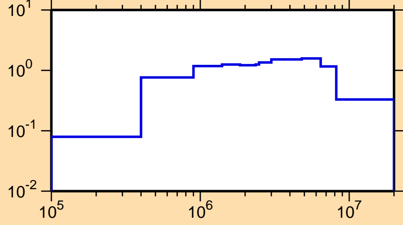
\sigma vs. E for ^{61}\text{Fe}(n,\text{inel.})
