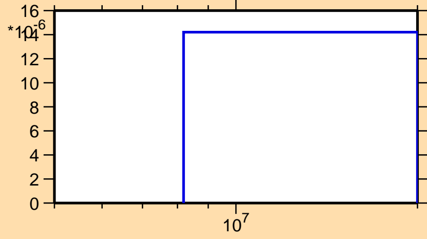
\sigma vs. E for ^{61}\text{Fe}(n,np)
