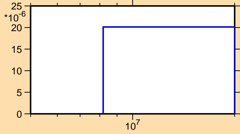
\sigma vs. E for ^{61}\text{Fe}(n,\alpha)
