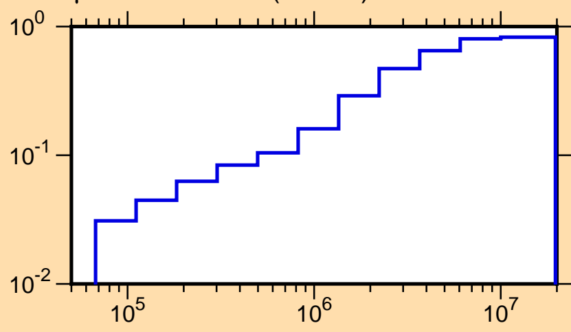
\mu vs. E for ^{62}\text{Fe}(\text{mt251})
