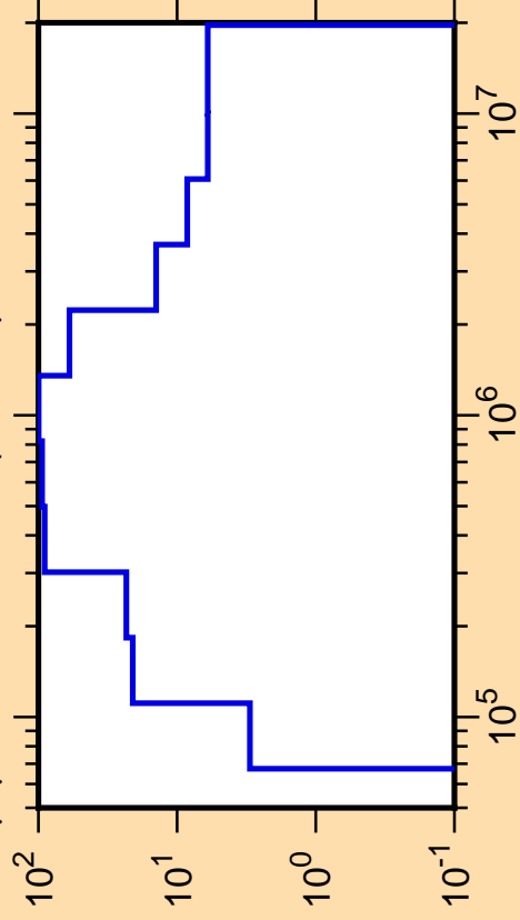
\Delta\mu/\mu vs. E for ^{62}\text{Fe}(\text{mt251})
